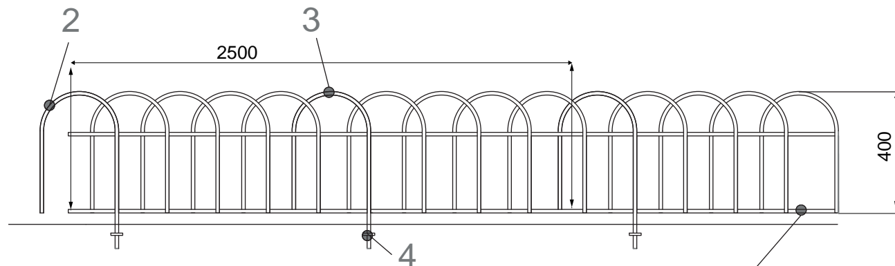
ALZADO PRINCIPAL
